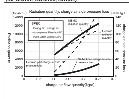
NISMO Intercooler performance data (for BNR32, BCNR33, BNR34)
